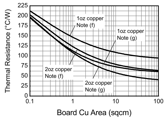
Thermal Resistance v Board Area
